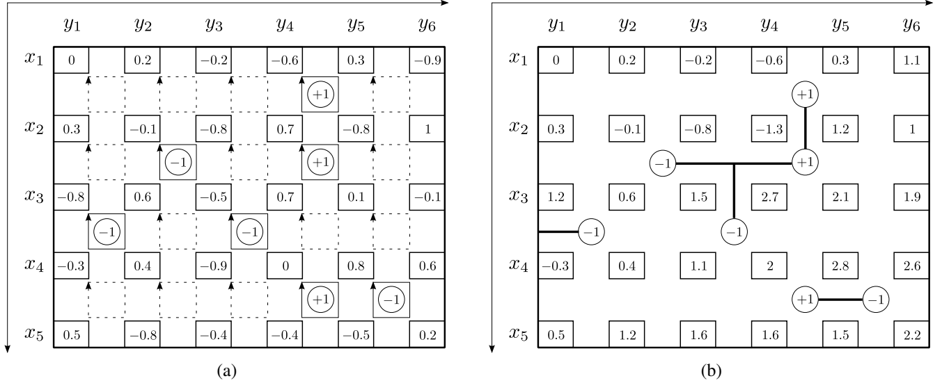
Fig. 1. Illustration of the idea of Goldstein's branch cut [20] for 2D phase unwrapping: (a) detection of every closed loop having a nonzero residue r_{i,j} = \pm 1 in (7) from given normalized wrapped phase \phi_{i,j}^W/\pi ( i = 1, 2, \dots, 5 and j = 1, 2, \dots, 6 ) and (b) construction of branches and the corresponding normalized unwrapped phase \phi_{i,j}/\pi ( i = 1, 2, \dots, 5 and j = 1, 2, \dots, 6 ).
