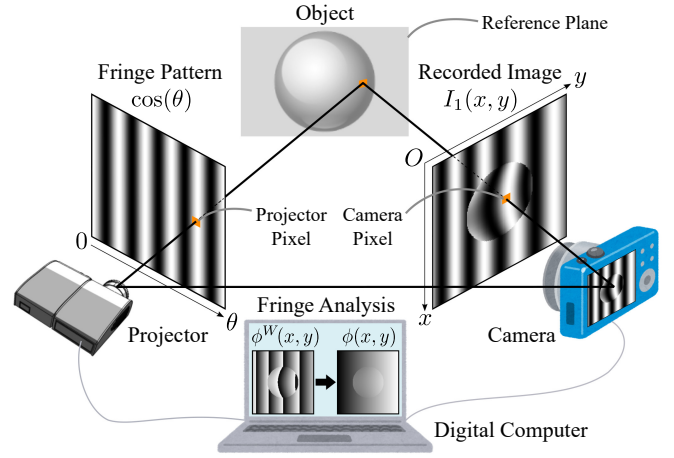
Fig. 3. Typical fringe projection profilometry system.
