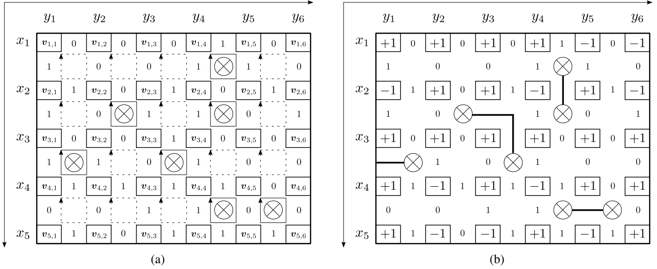
Fig. 2. Illustration of the idea of the proposed branch cut type sign estimator: (a) detection of every closed loop satisfying (12) by using the locally ideal sign changes c_{i,j}^{h,\min} and c_{i,j}^{v,\min} computed from v_{i,j} ( i = 1, 2, \dots, 5 and j = 1, 2, \dots, 6 ) and (b) constructions of branches, sign changes c_{i,j}^h and c_{i,j}^v , and the corresponding signs s_{i,j} ( i = 1, 2, \dots, 5 and j = 1, 2, \dots, 6 ).
