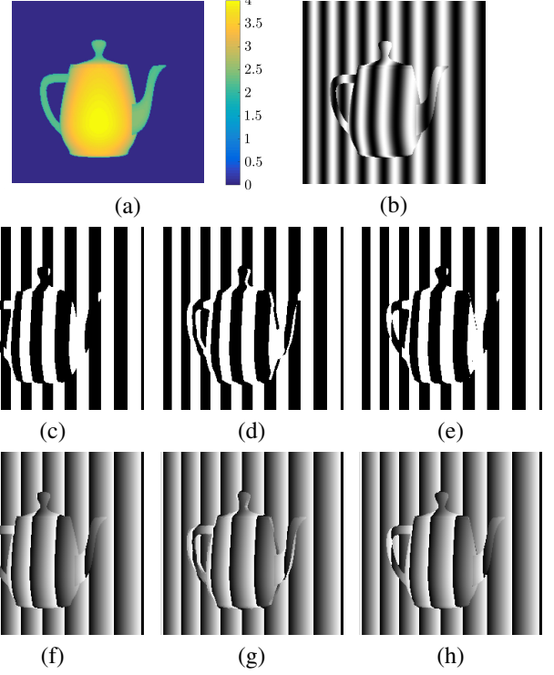
Fig. 5. Experimental results II: (a) object, (b) normalized fringe image I_{i,j} , (c) true signs s_{i,j} = \text{sgn}(\phi_{i,j}^W) (to be estimated), (d) signs estimated by [12], (e) signs estimated by the proposed branch cut, (f) true wrapped phase \phi_{i,j}^w , (g) wrapped phase based on (d), and (h) wrapped phase based on (e).
