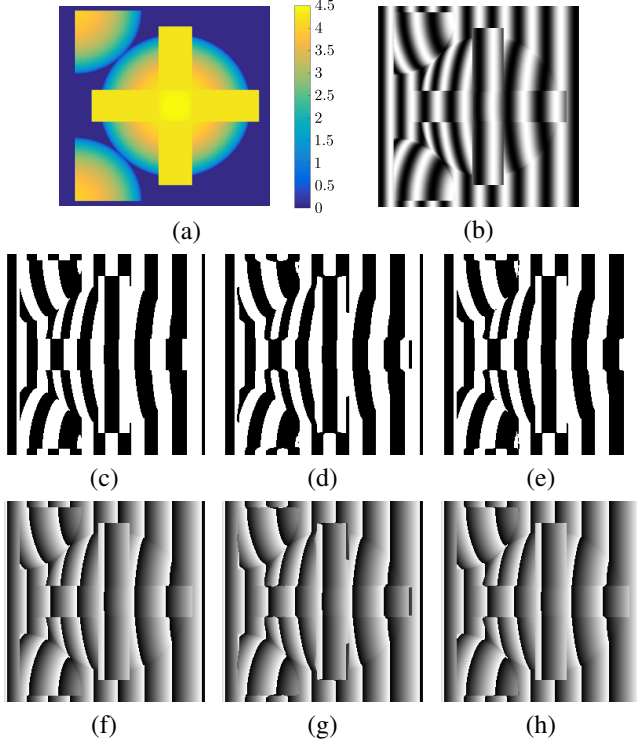
Fig. 4. Experimental results I: (a) object, (b) normalized fringe image I_{i,j} , (c) true signs s_{i,j} = \text{sgn}(\phi_{i,j}^W) (to be estimated), (d) signs estimated by [12], (e) signs estimated by the proposed branch cut, (f) true wrapped phase \phi_{i,j}^w , (g) wrapped phase based on (d), and (h) wrapped phase based on (e).
